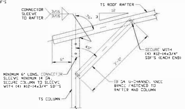
BOX EAVE RAFTER COLUMN CONNECTION DETAIL FOR HEIGHTS <= 12'-0"
