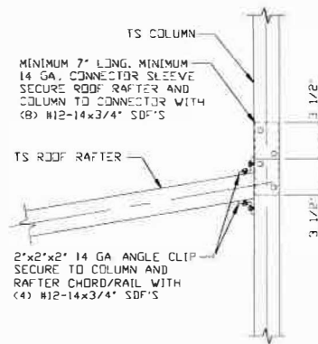
LEAN-TO RAFTER TO RAFTER COLUMN CONNECTION DETAIL FOR RAFTER SPANS ≤ 12'-0"
