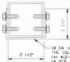
BRACE SECTION
