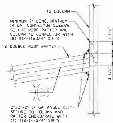
LEAN-TO RAFTER TO RAFTER COLUMN CONNECTION DETAIL FOR RAFTER SPANS 12'-0" < TO ≤ 16'-0"
